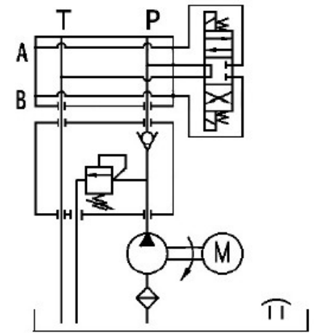
HYDRAULIC CIRCUIT
