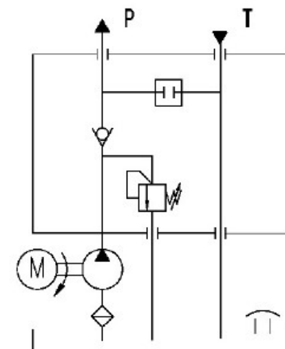
HYDRAULIC CIRCUIT
